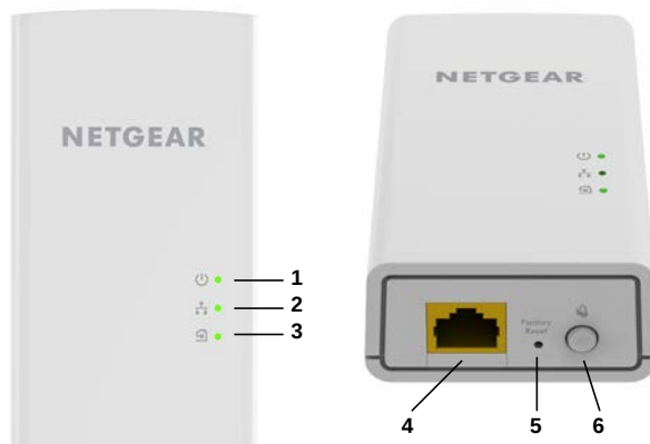
Figure 2. Hardware features
