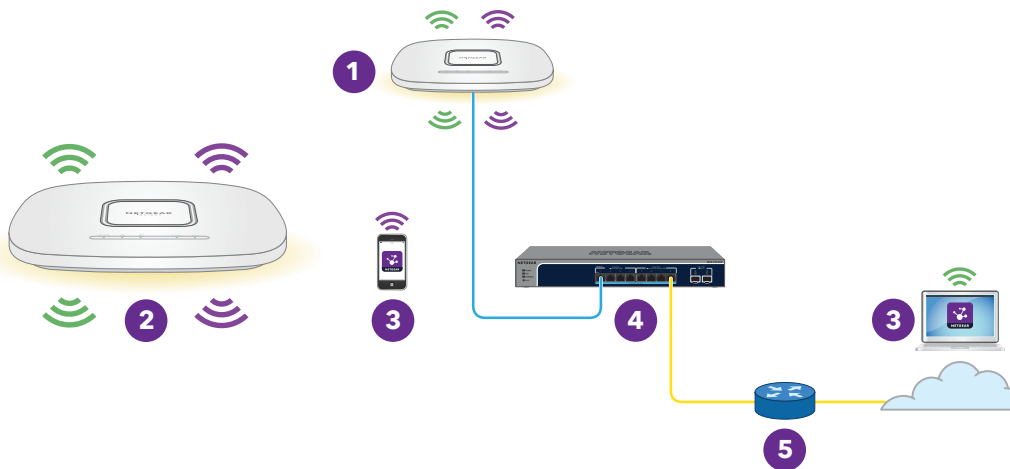
Figure 6. Mesh network with an extender access point and a wired root access point
