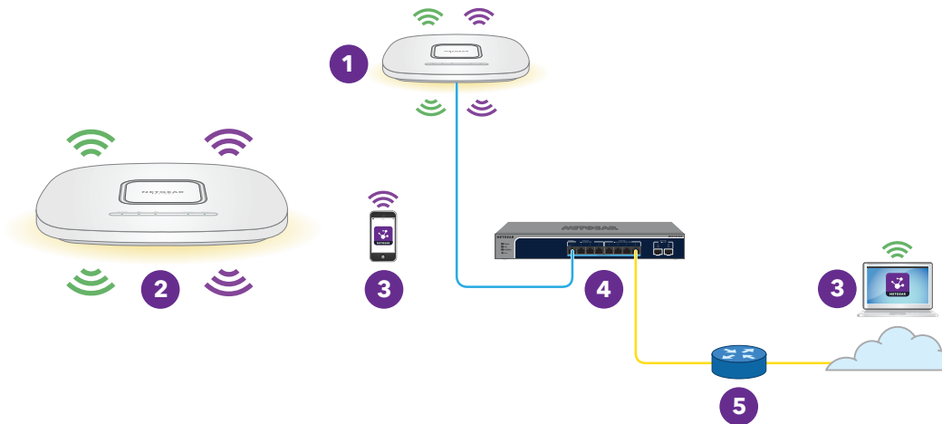
Figure 8. Connect the extender access point to a wired root access point
