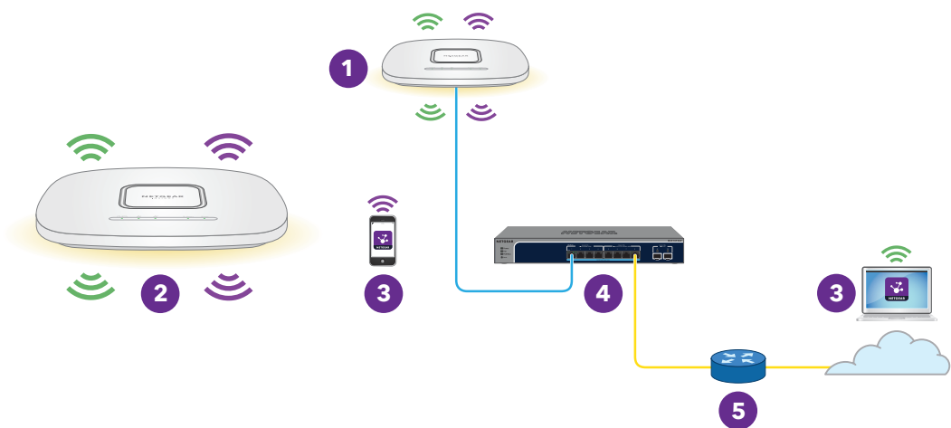
Figure 7. Connect the extender access point to a wired root access point
