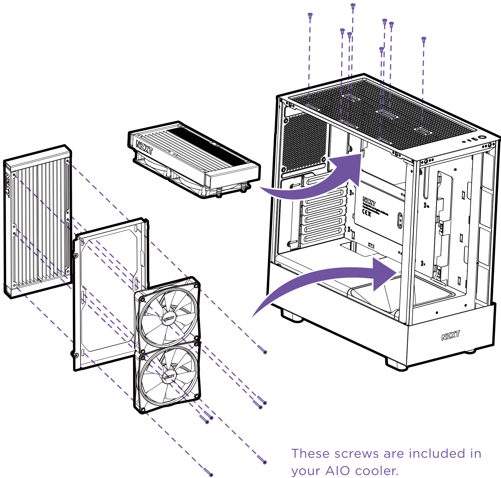
RADIATOR
