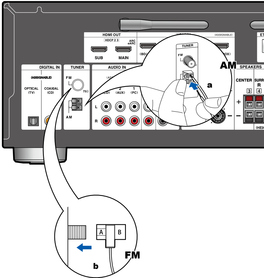
a AM loop antenna, b Indoor FM antenna
