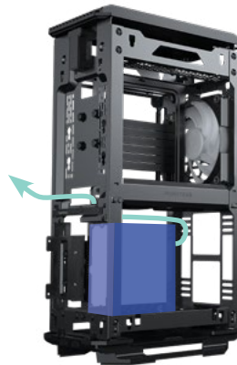
2. PRE-ROUTE CABLES TO THE OUTSIDE
