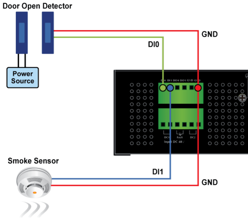
Figure 2-17 Wiring DIO and DI1 to Open Detector
