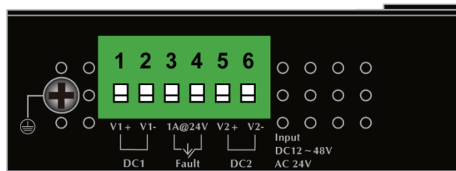
Figure 2-13: IGS-5225-4T2S Upper Panel
