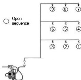
Section of flushing
