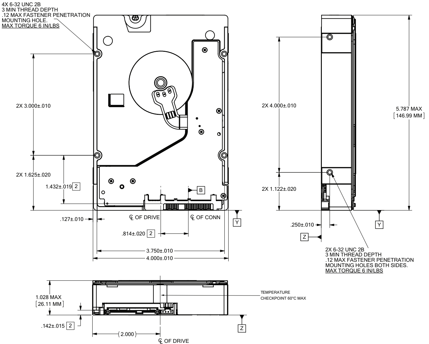
Figure 4. Mounting configuration dimensions (10TB & 8TB) models)
