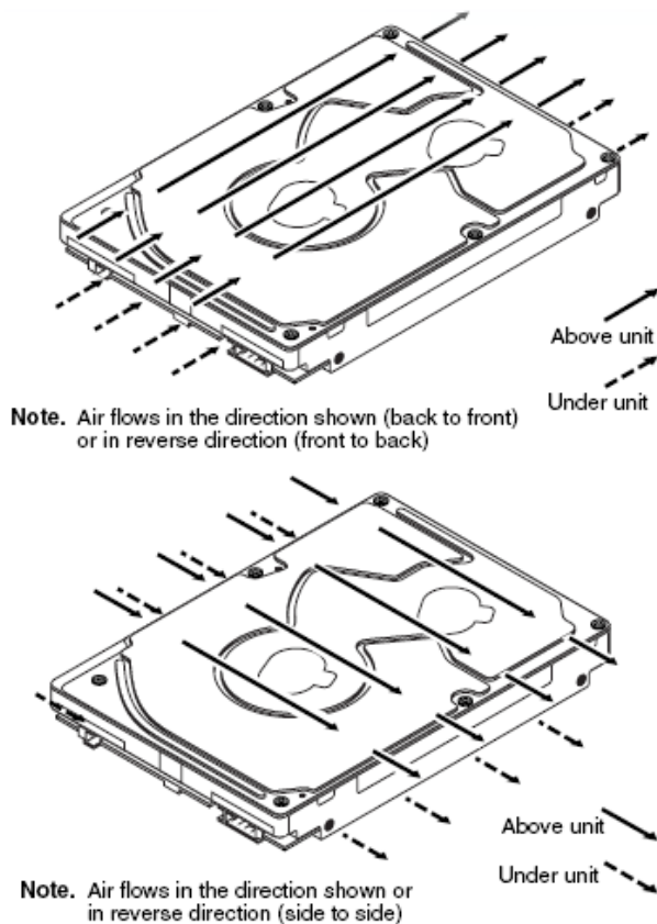
Figure 9. Air flow
