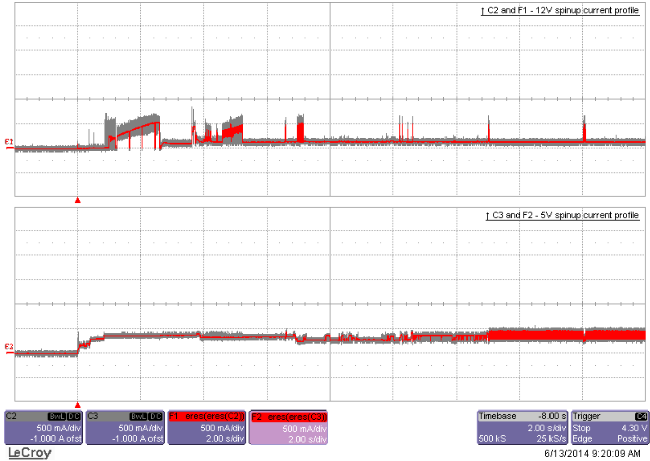
Figure 2. Current profiles for 1TB models
