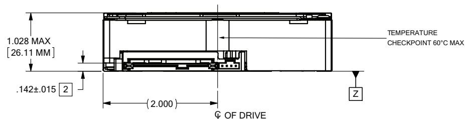
Figure 5. Mounting configuration dimensions (8TB & 6TB models)
