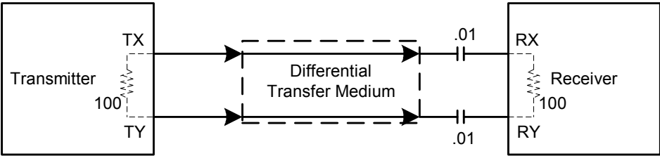
Figure 18. SAS transmitters and receivers
