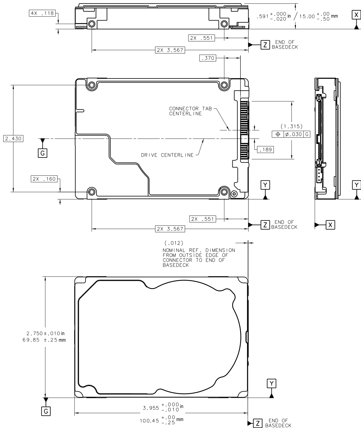
Figure 11. Dimensions
