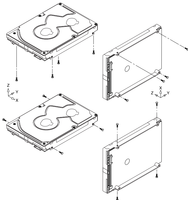
Figure 10. Recommended mounting
