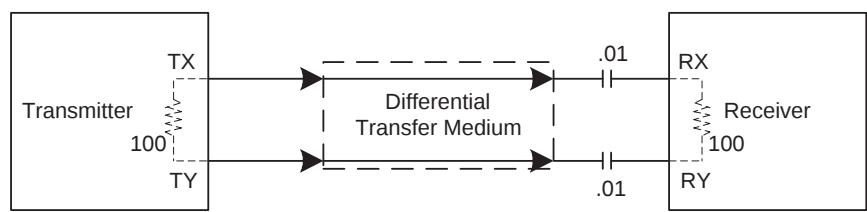
Figure 14. SAS transmitters and receivers
