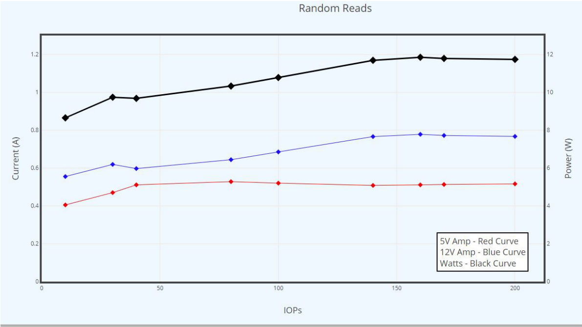
Figure 4. 6TB models (12Gb) DC current and power vs. input/output operations per second
