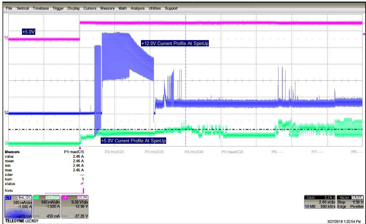
Figure 3. 2TB model current profiles
