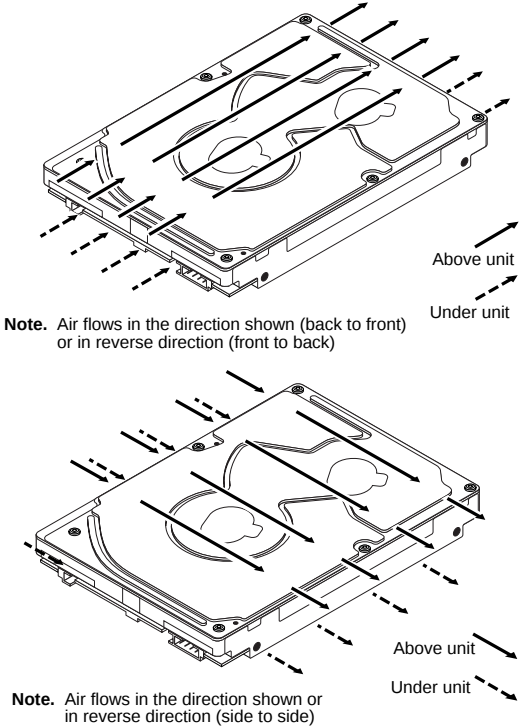
Figure 8. Air flow
