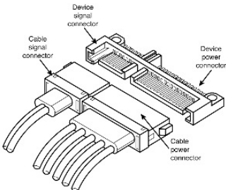
Figure 2. Attaching SATA cabling
