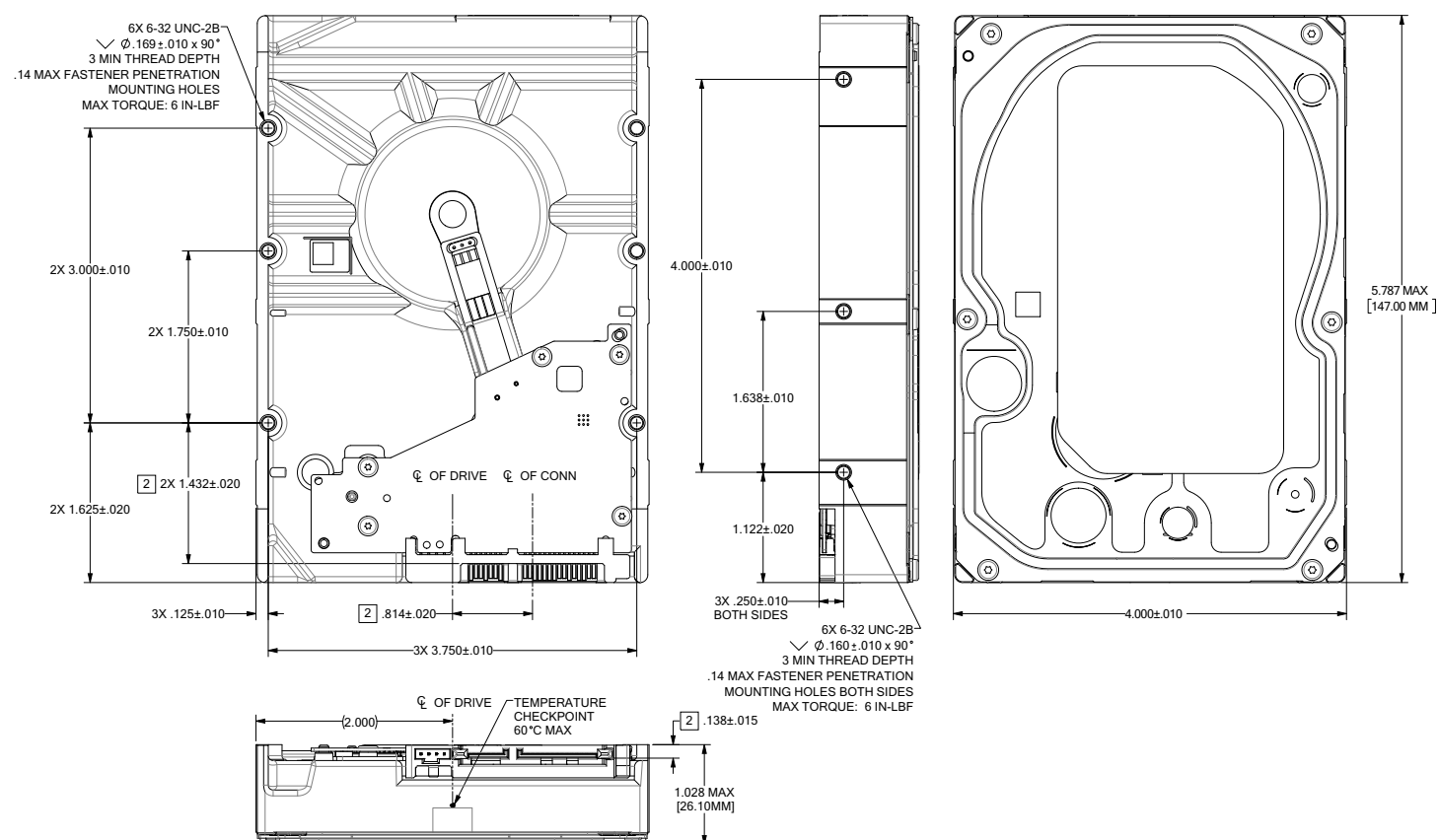
Figure 3. Mounting configuration dimensions 5-disk models
