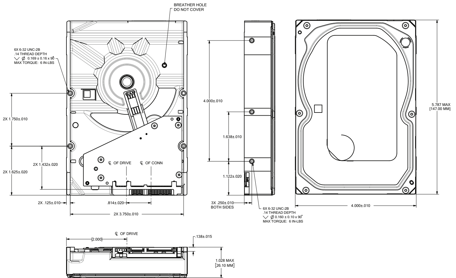
Figure 7. Mounting configuration dimensions 4TB and 2TB models
