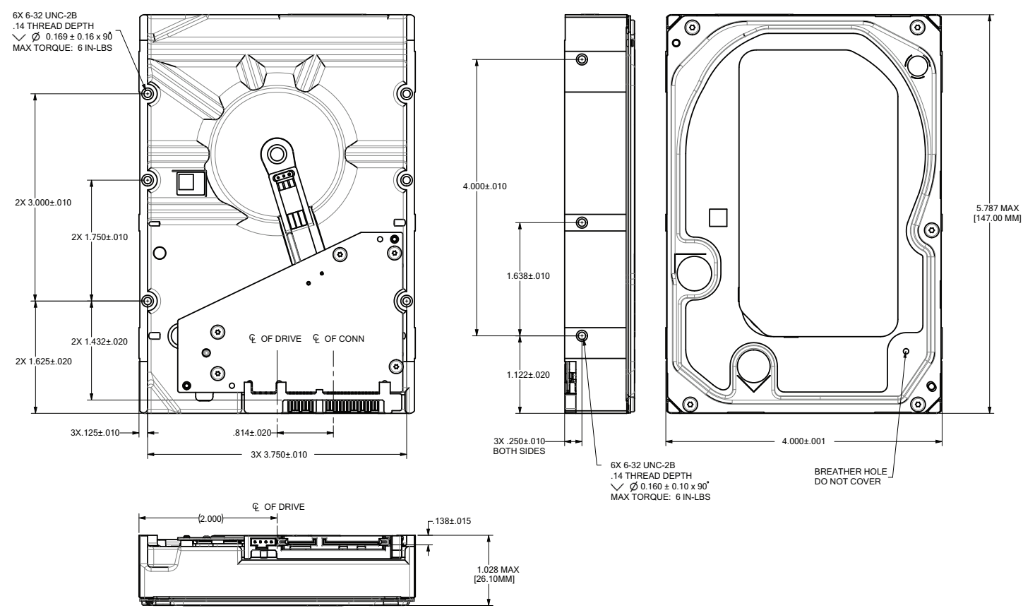
Figure 6. Mounting configuration dimensions 8TB and 6TB models
