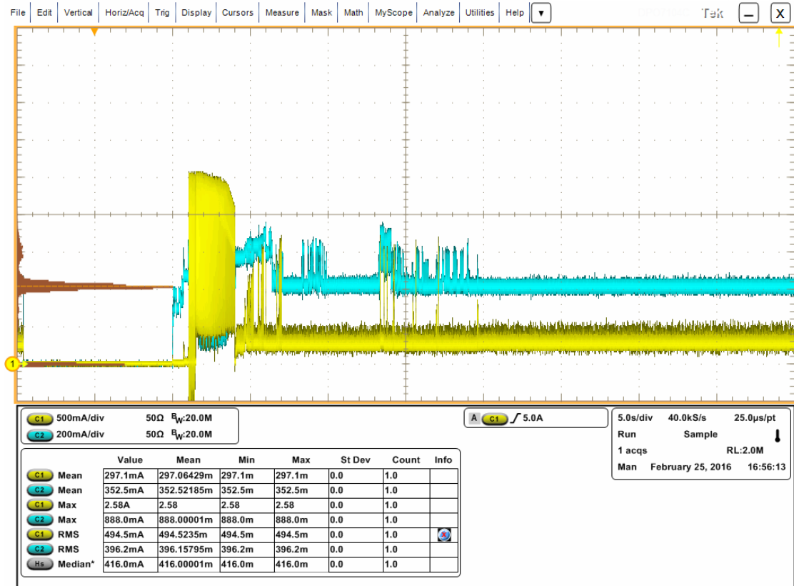
Figure 2. 2TB and 1TB models current profiles
