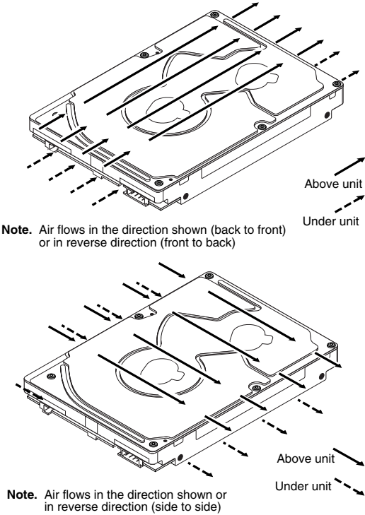
Figure 10. Air flow
