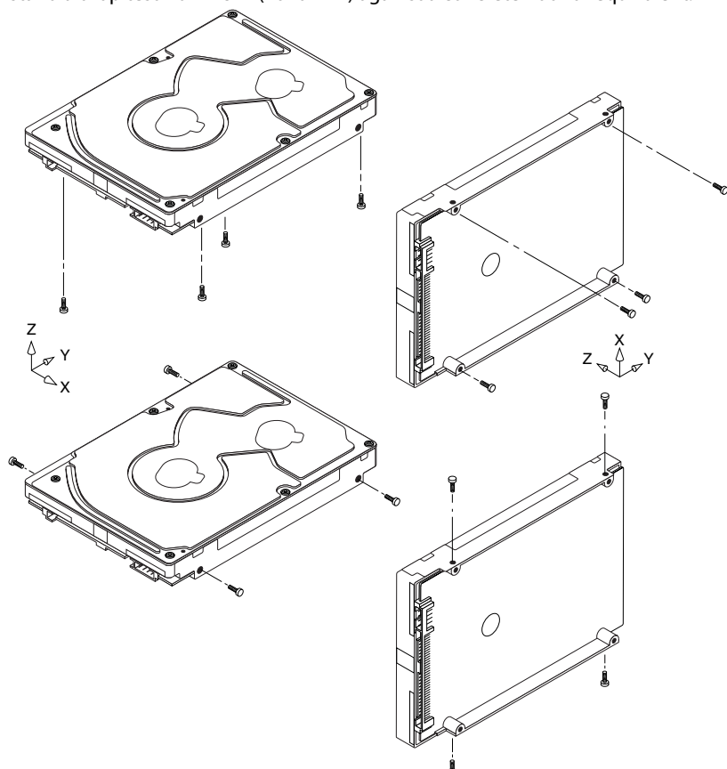
Figure 6. Recommended mounting
