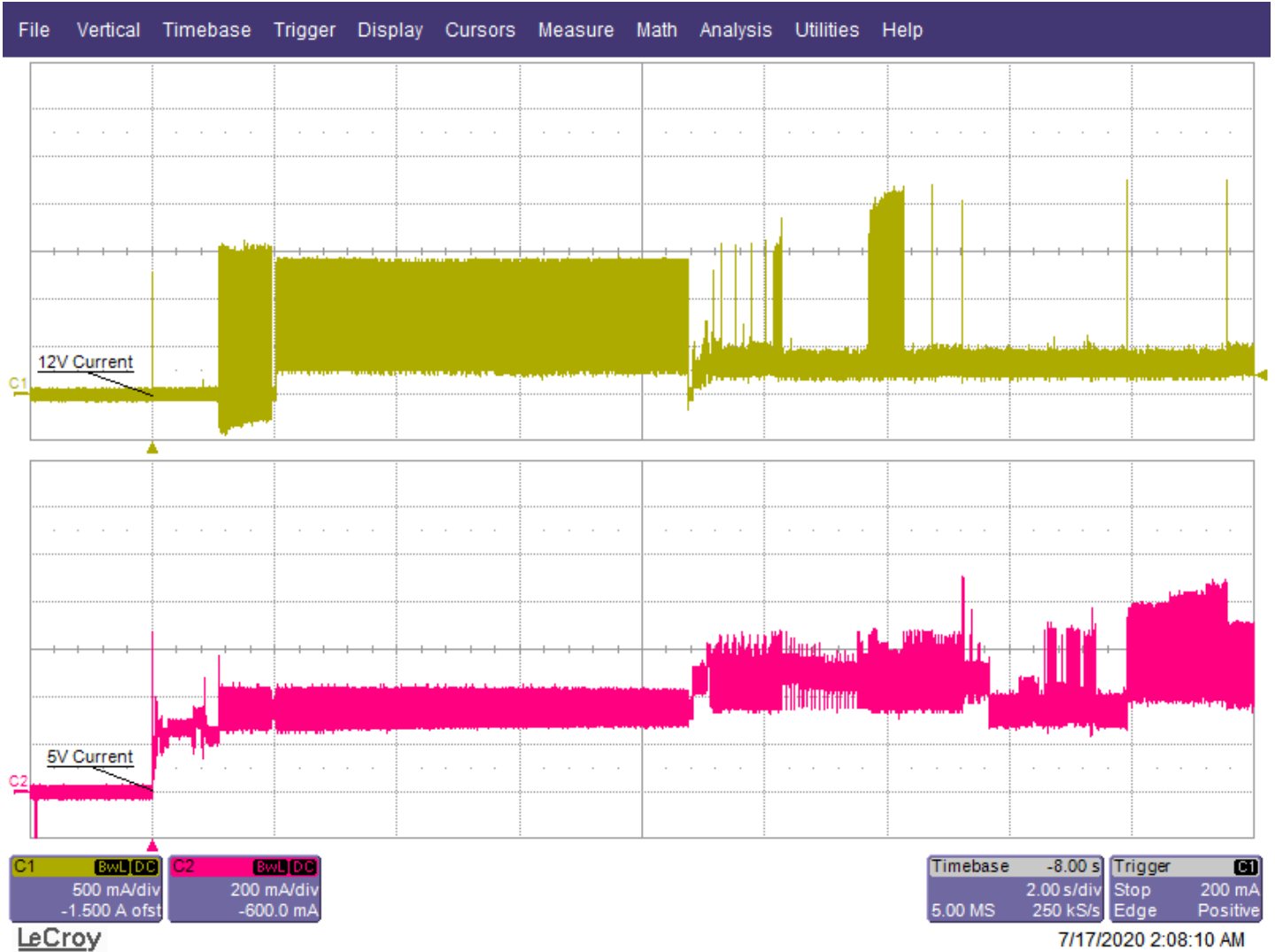
Figure 1. Typical 5V and 12V startup and operation current profiles (18TB and 16TB)
