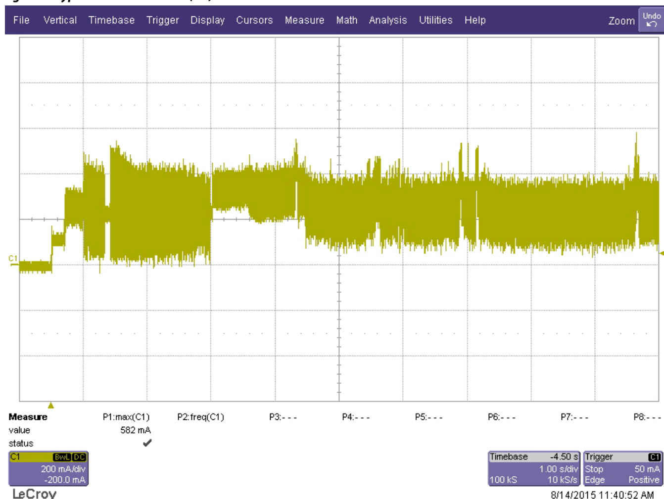
Figure 2 Typical Current Profiles (5V)
