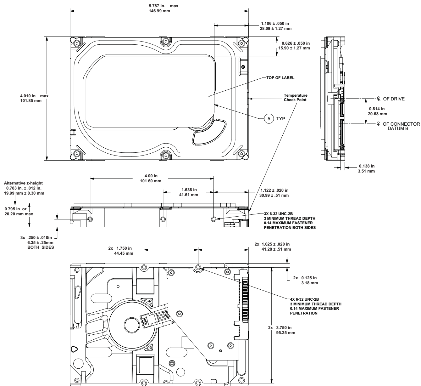
Figure 4 Mounting dimensions (1TB model)
