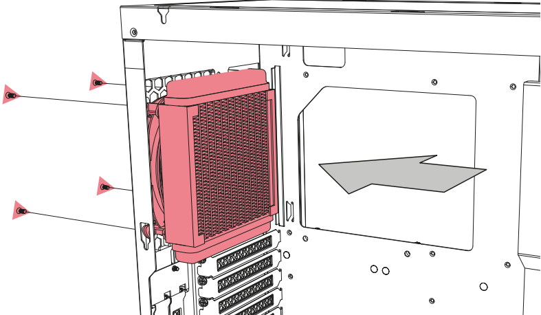
120 mm Radiator
