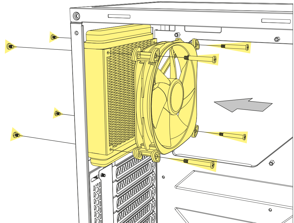
120 mm Radiator
