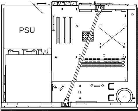
Power supply length limitation 140mm
