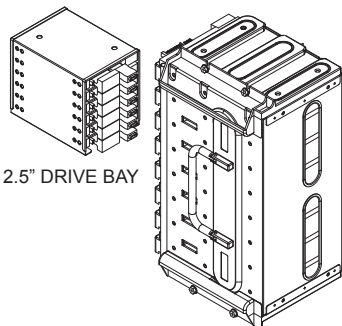
3.5" DRIVE BAY
