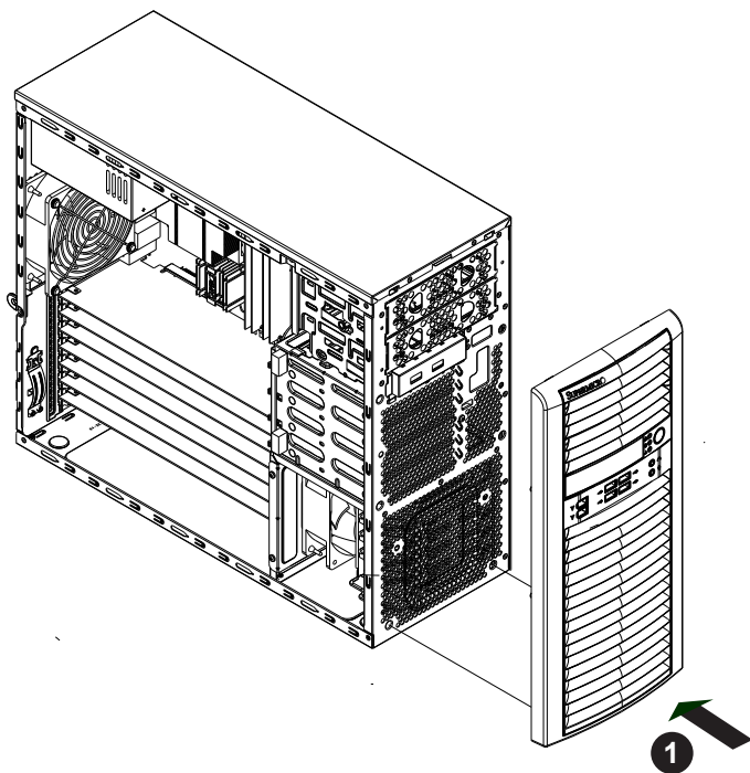
Figure 4-15. Installing the Front Bezel
