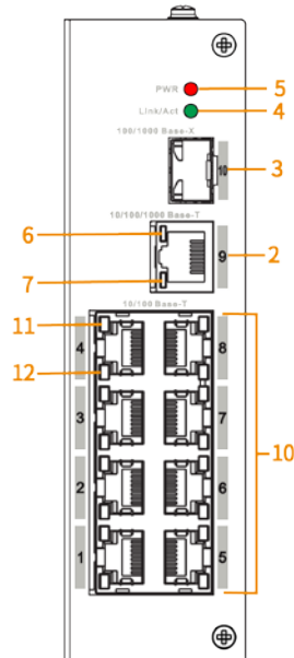
Figure 2-2 Front panel (without PoE)
