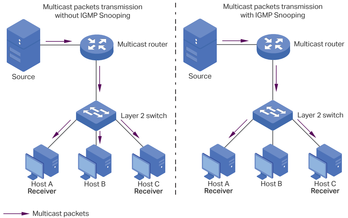
Figure 1-1 IGMP Snooping
