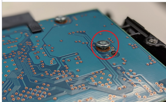
Loosened screw
