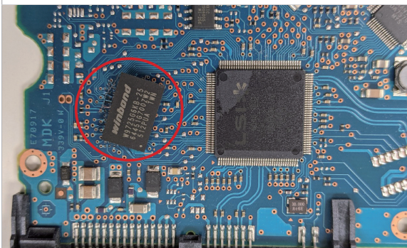
Out-of-shape/misaligned component
