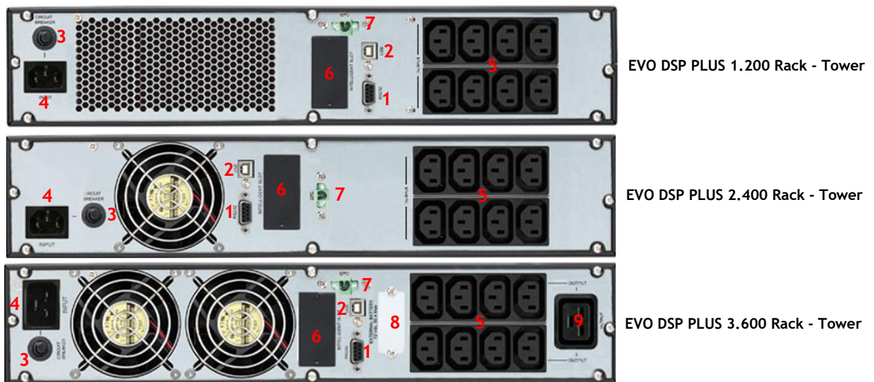
Figure 4 - Rear Side
