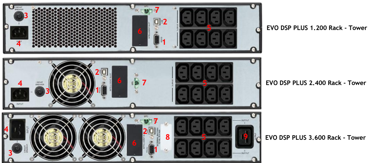
Figure 4 - Rear Side
