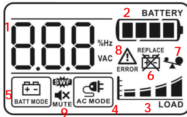
Figure 2 -LCD Display
