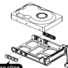
Locking clips
