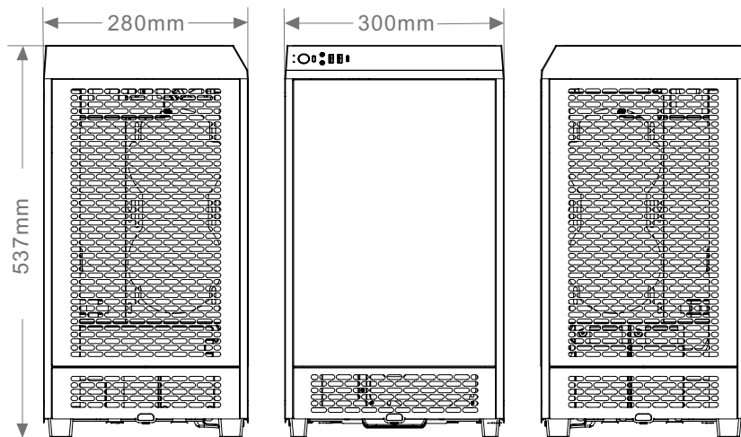
Chassis dimension
