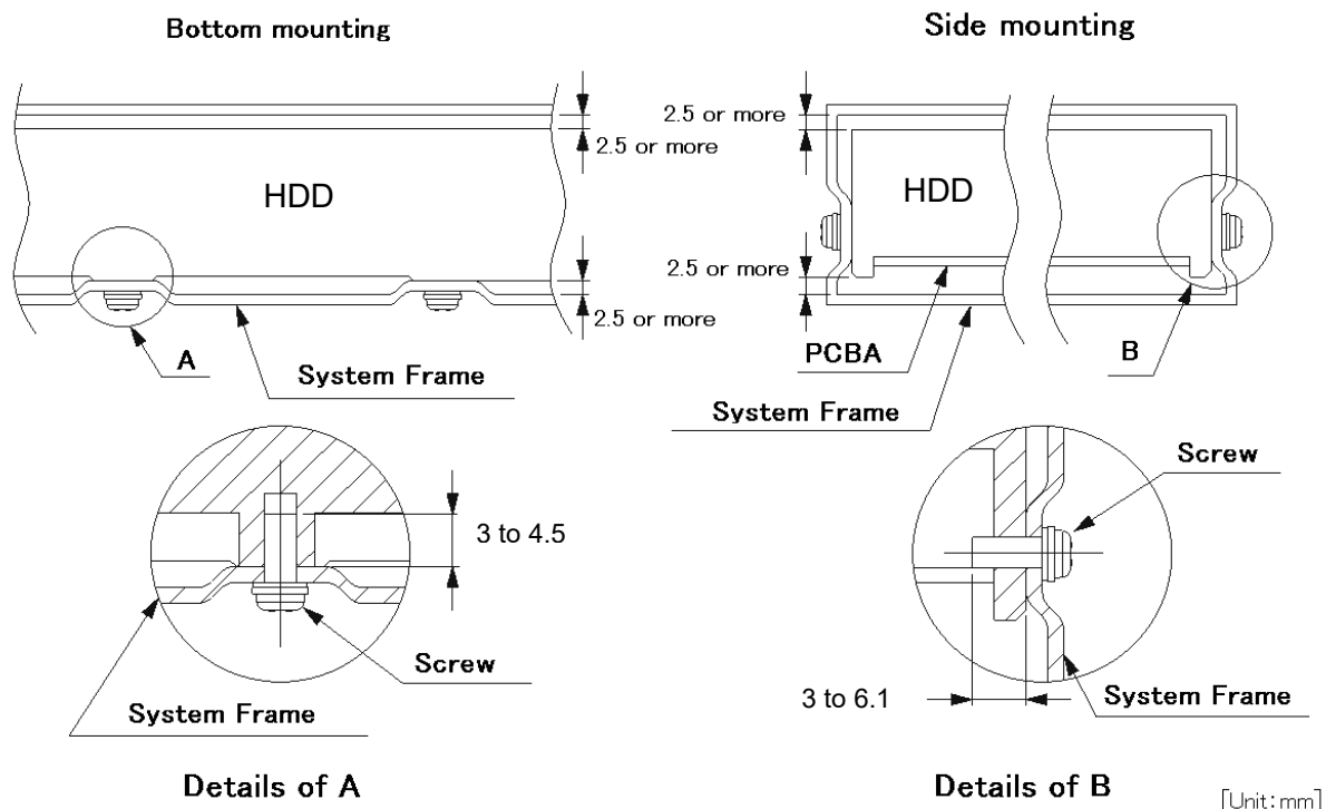
Figure 3.3 Mounting frame structure example
