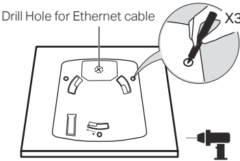
Drill Hole for Ethernet cable
