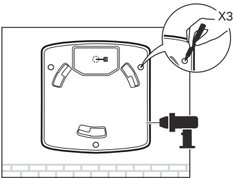
M3×28 Plastic Wall Anchors (Qty.3)
