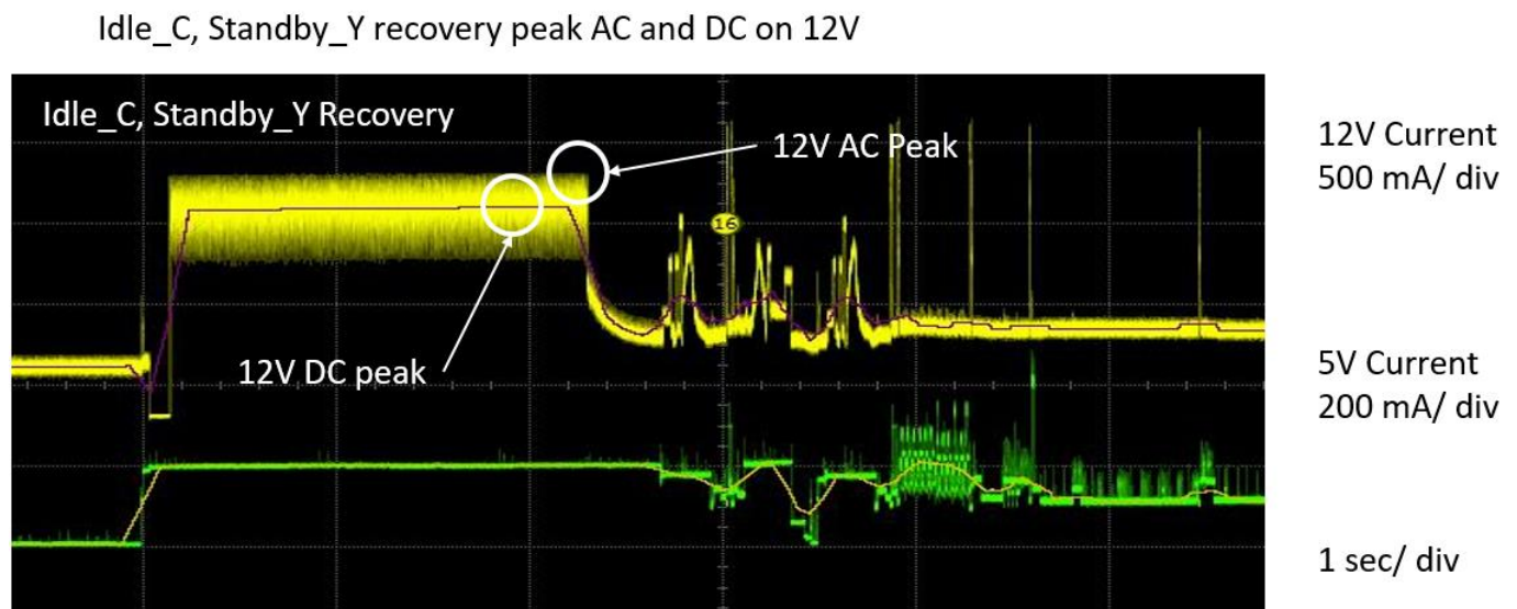
Figure 8 Idle_C Standby_Y, Recovery Current Waveform
