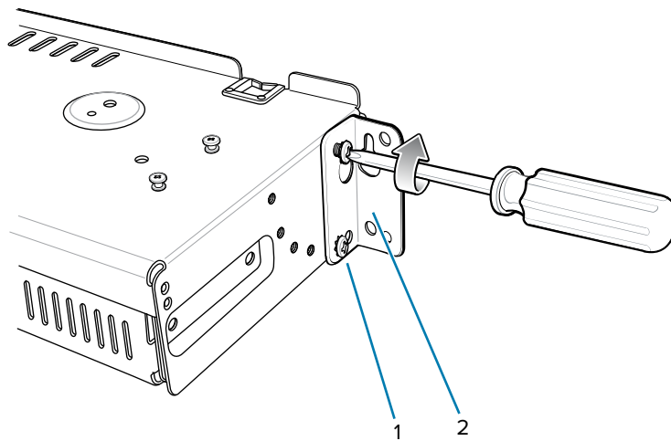
Figure 36 Flange Horizontal Position (5-Slot Cradles)
