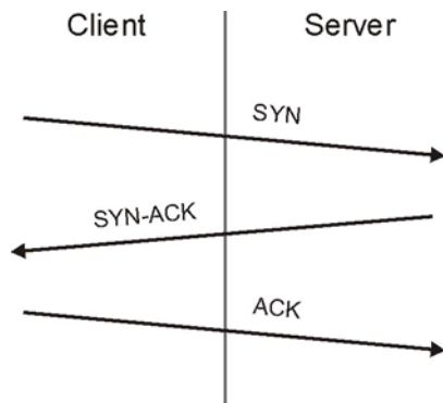
Figure 89 Three-Way Handshake
