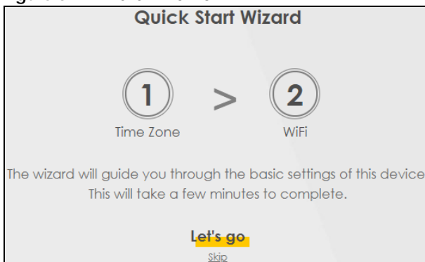
Figure 37 Wizard – Home
