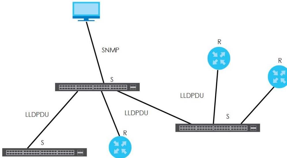
Figure 152 LLDP Overview
