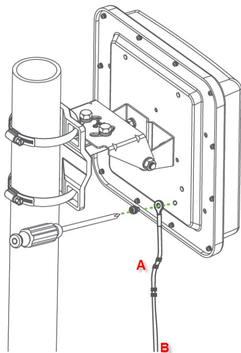
Figure 16 Grounding Example
