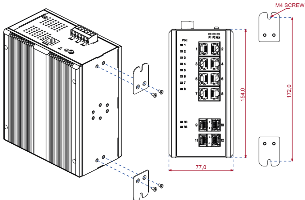
Figure 4 RGS200-12P Series Wall Mounting
