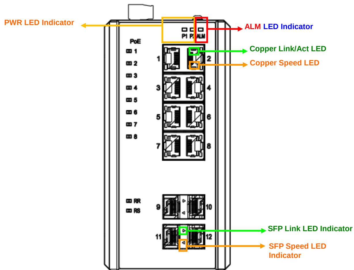
Figure 11 LED Indicators
