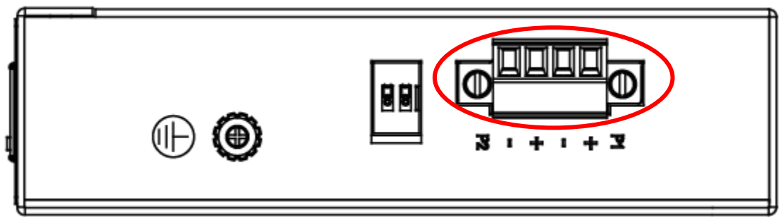
Figure 7 RGS100-5P Series Power Connections
