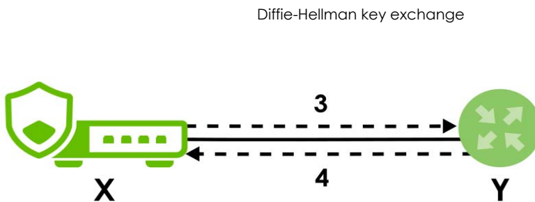
Figure 153 IKE SA: Main Negotiation Mode, Steps 3 - 4: DH Key Exchange
