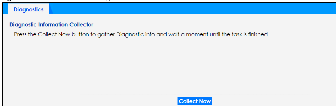
Figure 151 Maintenance > Diagnostics
