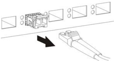
Figure 18 Removing the Fiber Optic Cables
